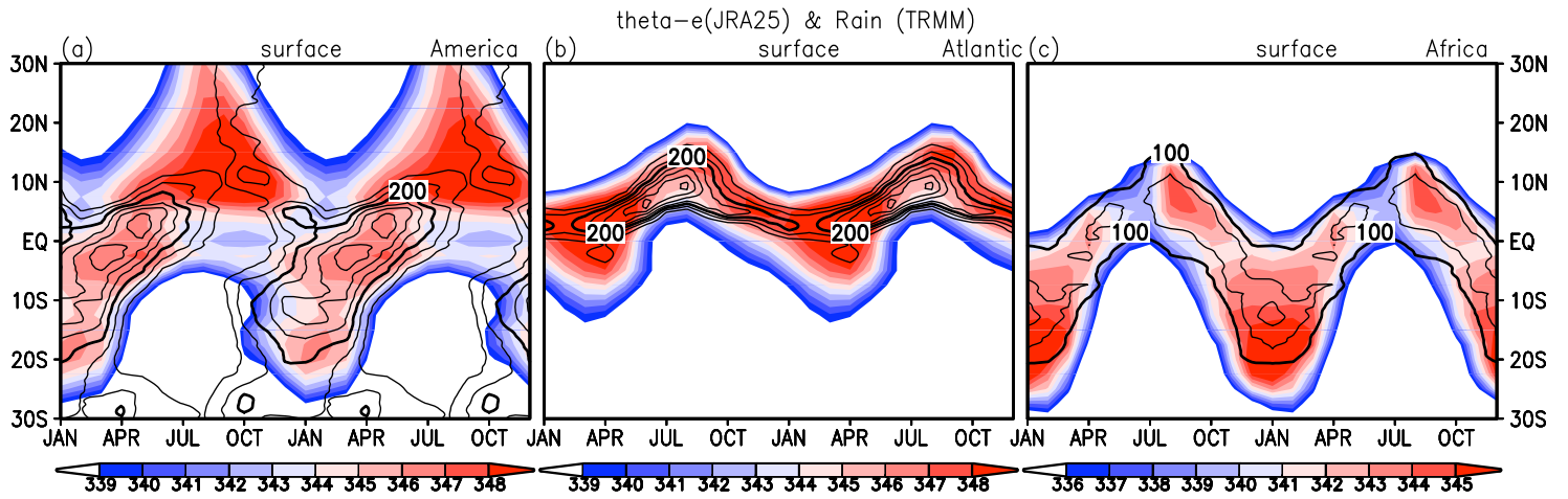
Figure 1 Latitude-time sections of rainfall (contour at 50 mm month -1 intervals) based on the TRMM 3B43 product and JRA25 equivalent potential temperature at the surface (colors in K) in (a) the South American (60-50°W), (b) Atlantic (20-10°W), and (c) African (20-30°E) sectors. Note that two annual cycles are presented. The longitudinal bands are chosen to avoid high orography of the Andes and African Rift Valley. The Atlantic (African) sector is all ocean (land).
