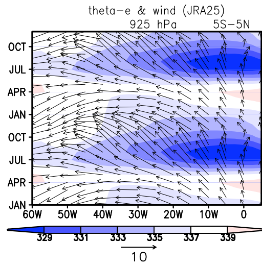
Figure 3 A longitude-time section of JRA25 equivalent potential temperature (colors in K) and wind velocity (arrows in \text{ms}^{-1} ) at 925hPa averaged over the 5°S-5°N band.
