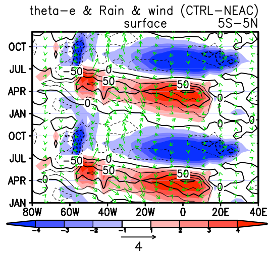
Figure 7 A longitude-time section of differences equivalent potential temperature (colors in K), wind velocity (arrows in \text{m s}^{-1} ) and rainfall (contours at 25 \text{ mm month}^{-1} intervals) at the surface averaged latitudinally for 5^{\circ}\text{S} - 5^{\circ}\text{N} between the CTRL and the NEAC experiments.
